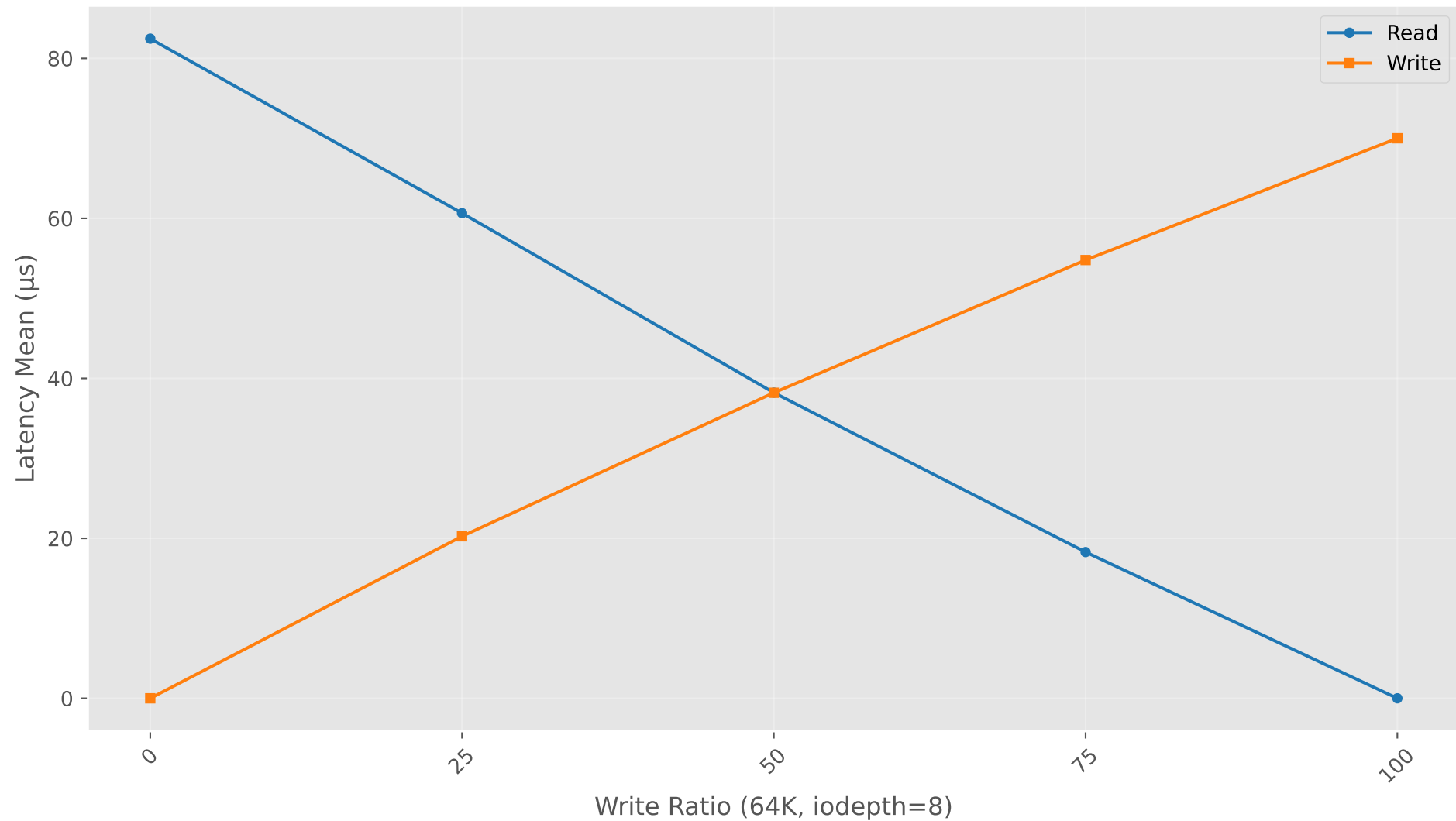
Latency Mean vs Write Ratio (64K, iodepth=8)
